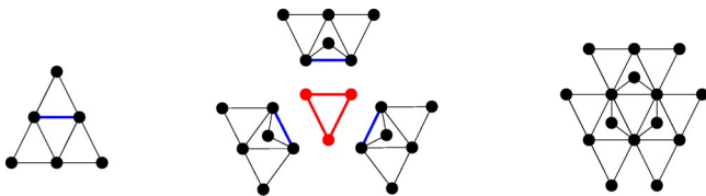
FIG. 2. (Color online) Recursive construction of K(2,t) . We glue a native (or initial) clique of a K(2,t-1) on each 2-clique of K_3 to construct K(2,t) . In this figure we obtain K(2,3) from three copies of K(2,2) as follows. The graph at the left is K(2,2) with its native 2-clique (the thick edge). Three copies of K(2,2) are glued by their natives 2-cliques to each of the three 2-cliques of K_3 (center) resulting in K(2,3) (right).
