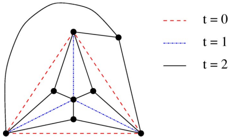
FIG. 1. (Color online) First stages of a growing recursive clique tree K(3,t) . K(3,0) is the complete graph or clique K_3 (the triangle with thick edges). At each step a vertex is connected to each of existing K_3 . Therefore at t=1 only one vertex is added, but at t=2 , four new vertices should be connected to the four different cliques K_3 .
